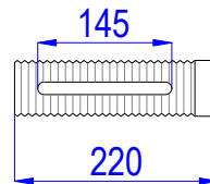
Prop Collar
