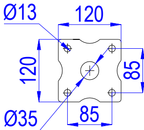
Top and Bottom Prop Plate
